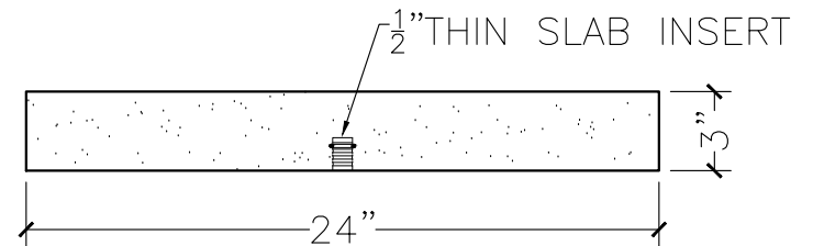
SECTION VIEW
