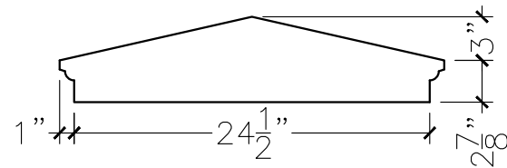
SECTION VIEW
