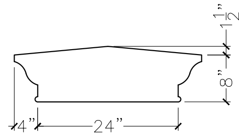
SECTION VIEW
