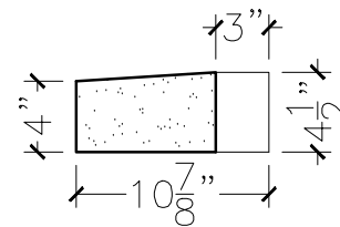
SECTION VIEW
