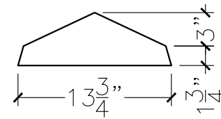
SECTION VIEW
