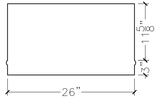
SECTION VIEW
