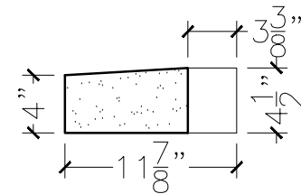
SECTION VIEW
