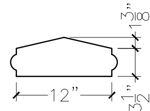
SECTION VIEW
