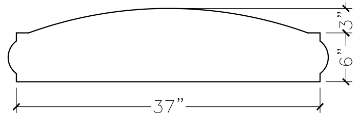
SECTION VIEW
