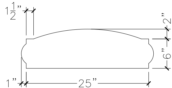
SECTION VIEW
