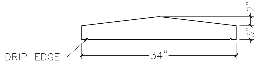
SECTION VIEW
