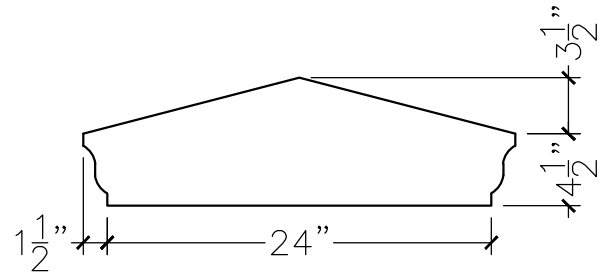
SECTION VIEW
