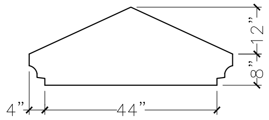
SECTION VIEW
