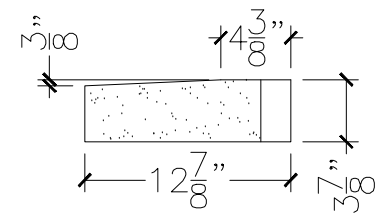
SECTION VIEW
