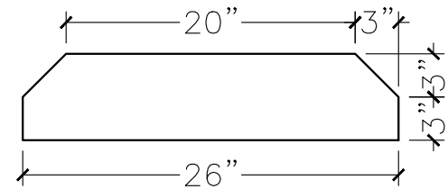
SECTION VIEW
