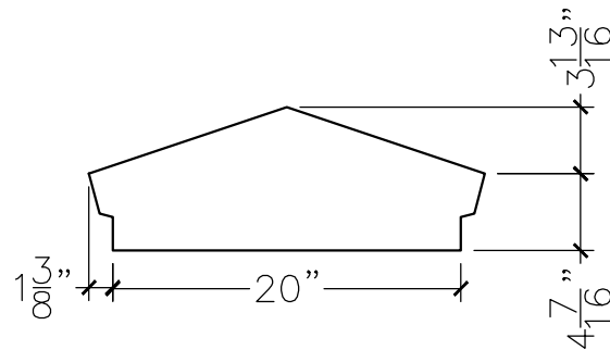
SECTION VIEW
