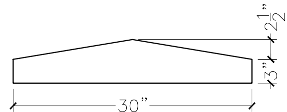
SECTION VIEW
