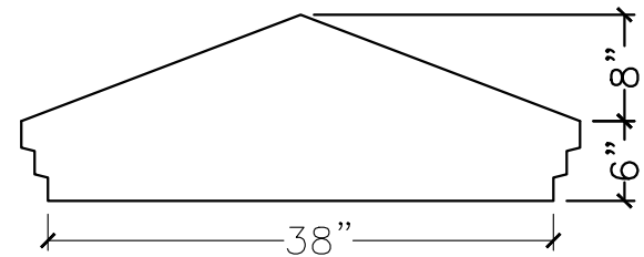
SECTION VIEW
