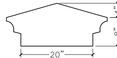
SECTION VIEW
