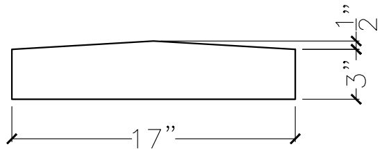
SECTION VIEW
