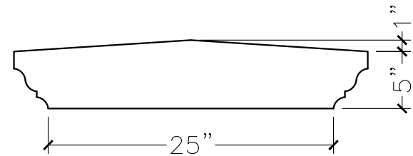
SECTION VIEW
