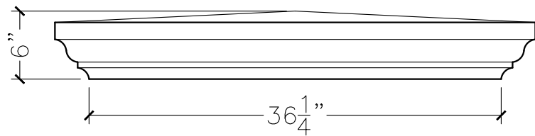
FRONT VIEW
