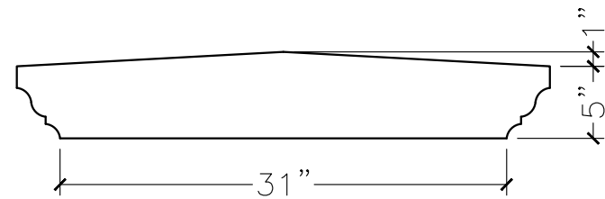
SECTION VIEW
