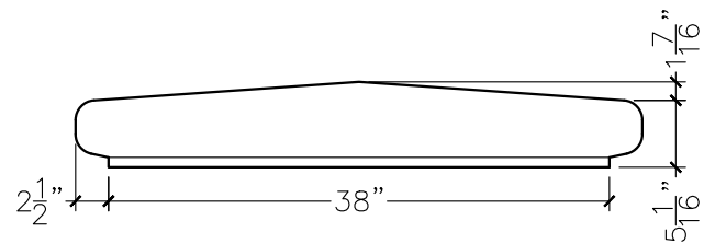
SECTION VIEW
