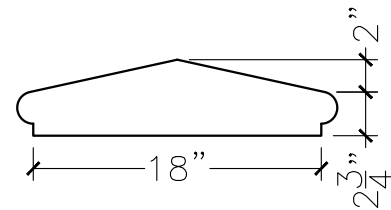
SECTION VIEW
