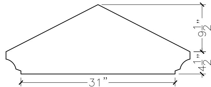
SECTION VIEW
