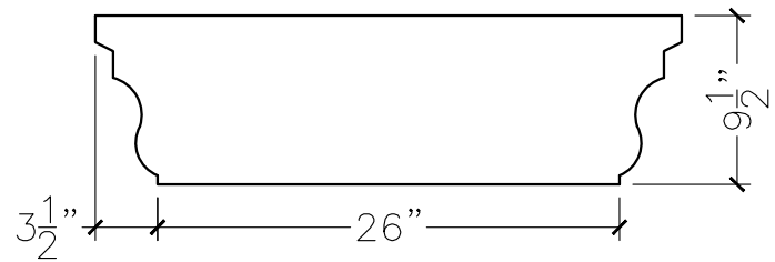
SECTION VIEW
