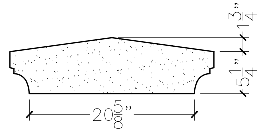
SECTION VIEW
