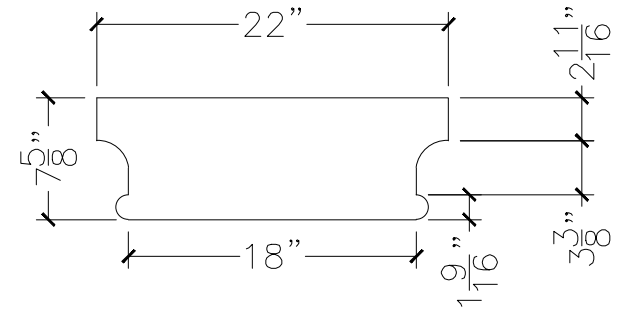
SECTION VIEW
