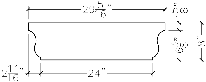
SECTION VIEW
