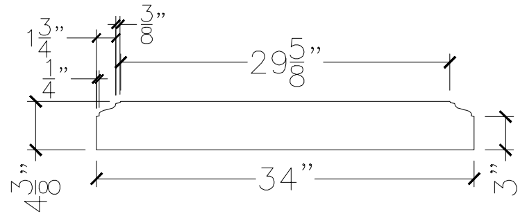
SECTION VIEW
