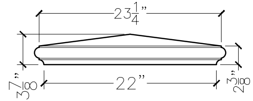
SECTION VIEW
