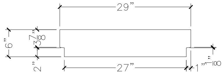
SECTION VIEW
