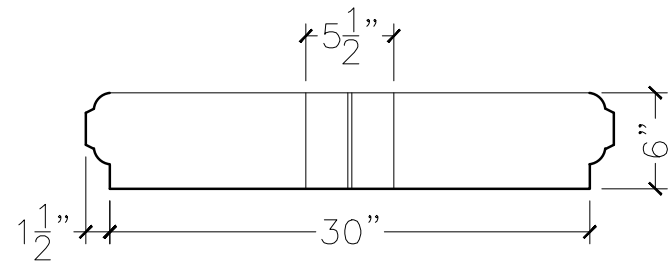
SECTION VIEW
