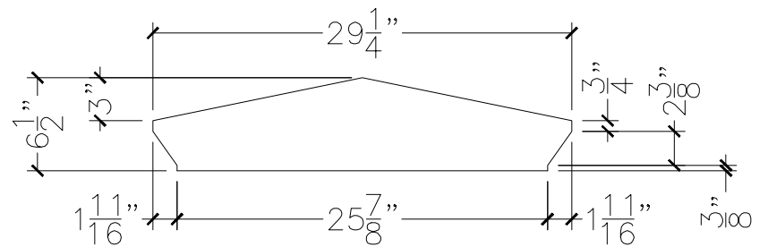
SECTION VIEW
