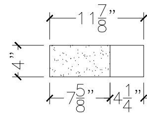
SECTION VIEW
