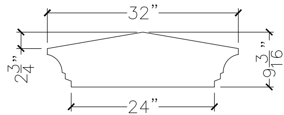
SECTION VIEW
