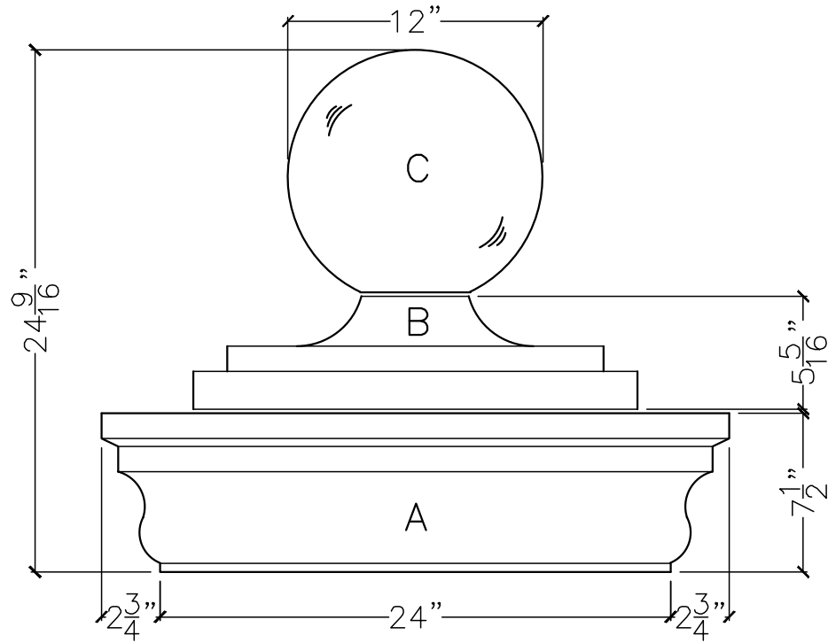
FRONT VIEW
