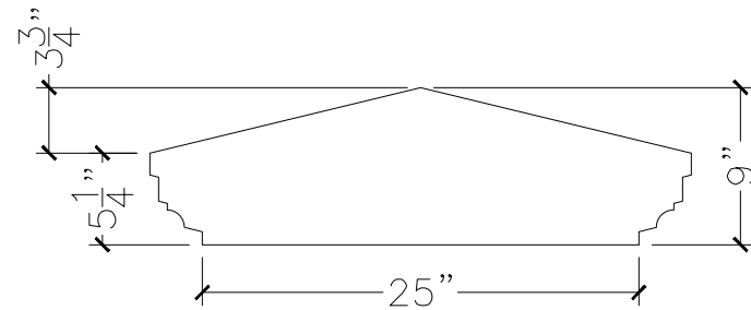
SECTION VIEW
