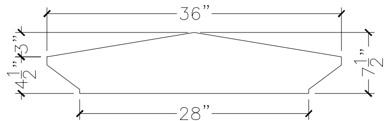
SECTION VIEW
