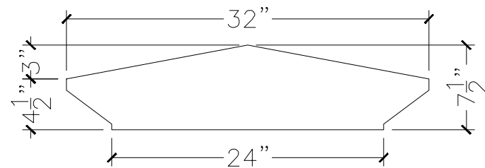
SECTION VIEW
