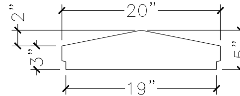
SECTION VIEW
