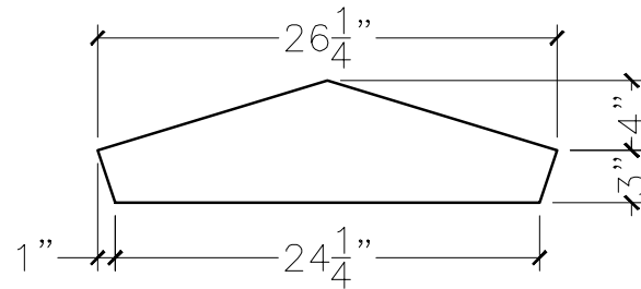
SECTION VIEW
