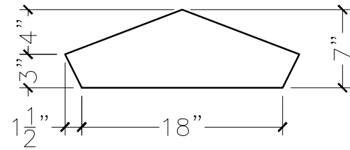
SECTION VIEW
