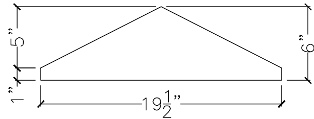
SECTION VIEW
