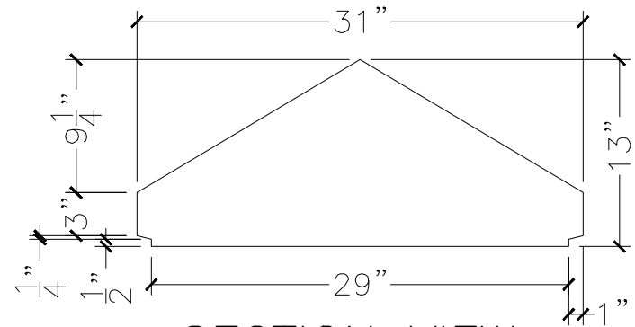
SECTION VIEW
