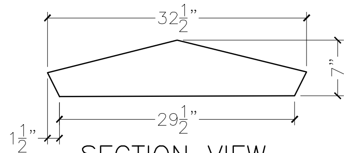
SECTION VIEW
