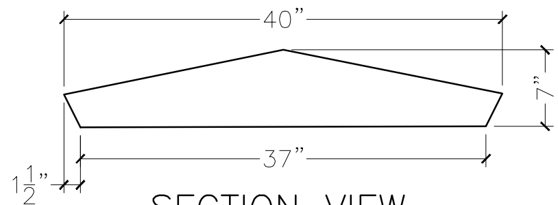
SECTION VIEW
