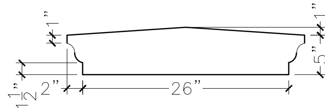
SECTION VIEW
