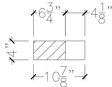
SECTION VIEW
