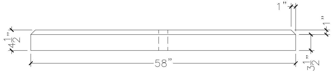
FRONT VIEW
